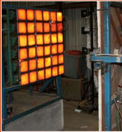
NFPA 268 test apparatus during a heat flux calibration. This method is used to determine the ignitability of exterior building products by exposure to a predefined heat flux in the presence of a pilot ignition source.
