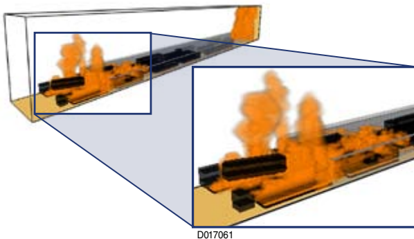
To evaluate thermal conditions during a truck fire event, computational fluid dynamics was used to calculate gas and tunnel wall temperatures.
